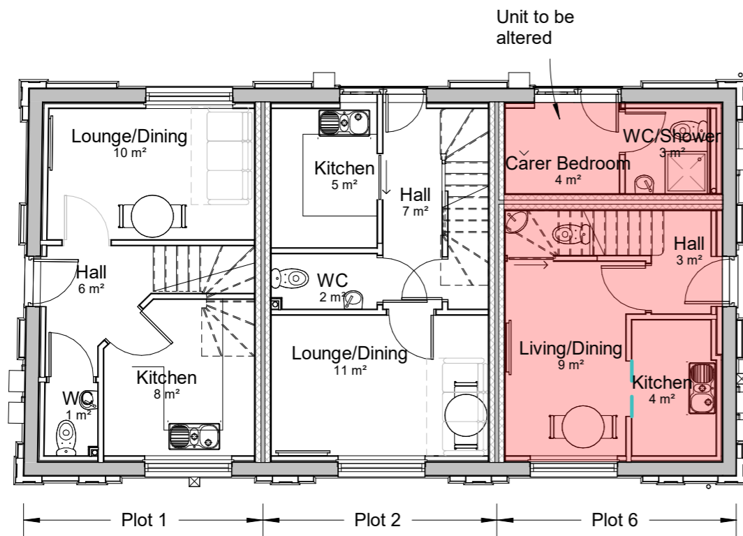
Ground Floor Plan (Planning) 1 : 100
