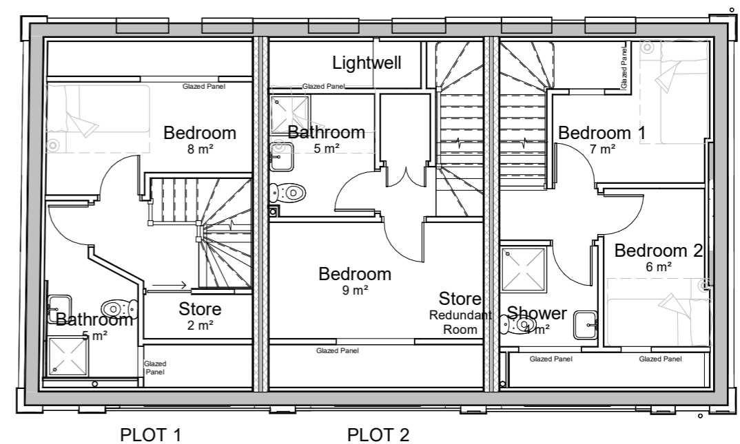
First Floor Plan (Planning) 1 : 100
