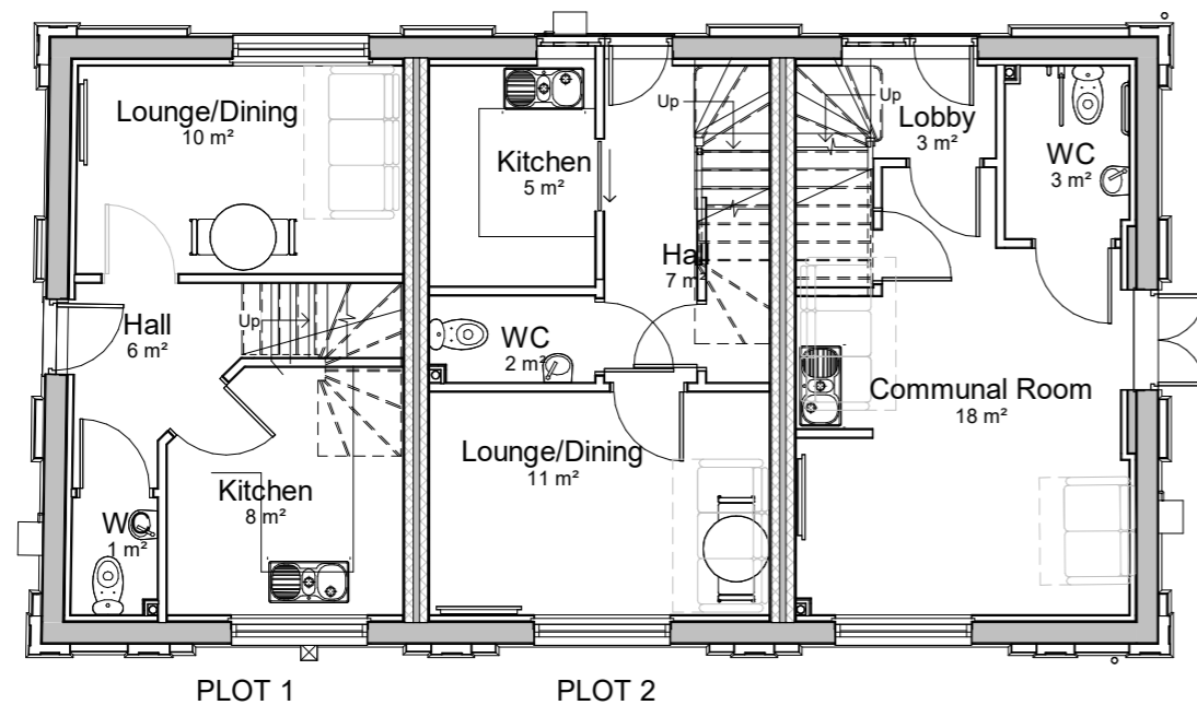
Ground Floor Plan (Planning) 1 : 100
